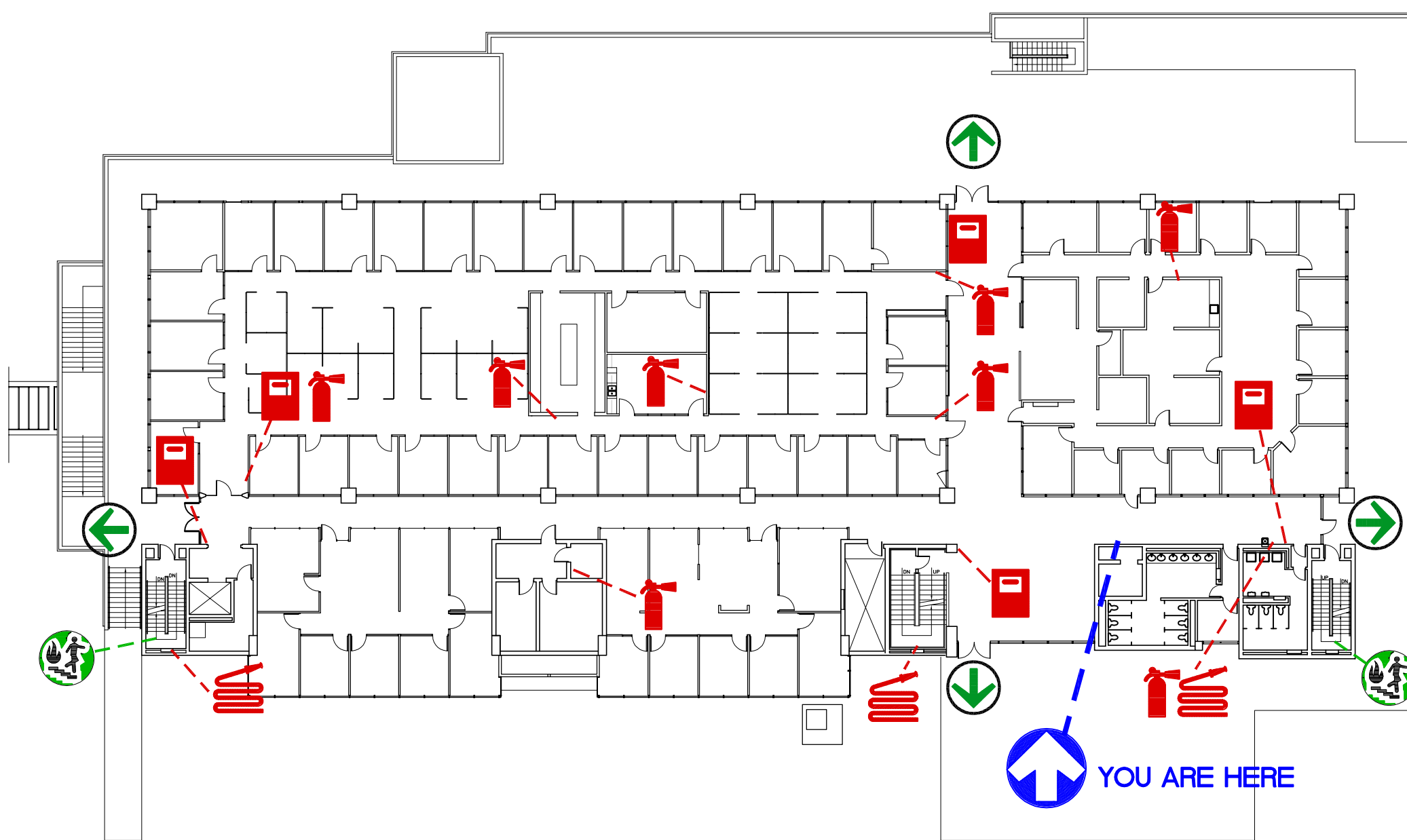
SECOND FLOOR PLAN(SOUTH) LEVEL 13 SCALE : NTS
